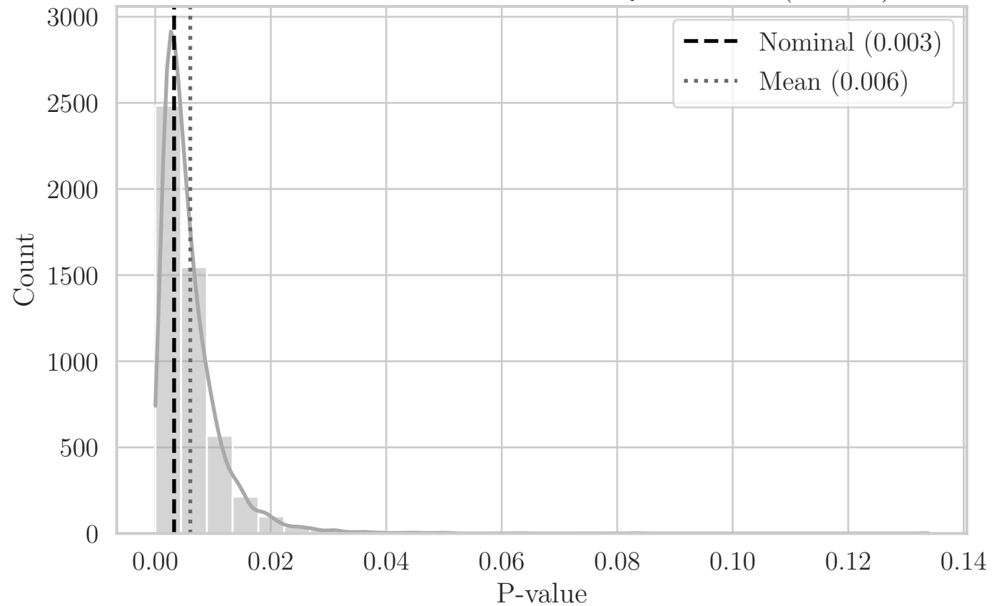
MC Distribution of P-values for QRS T-Dist (F2 XY)
