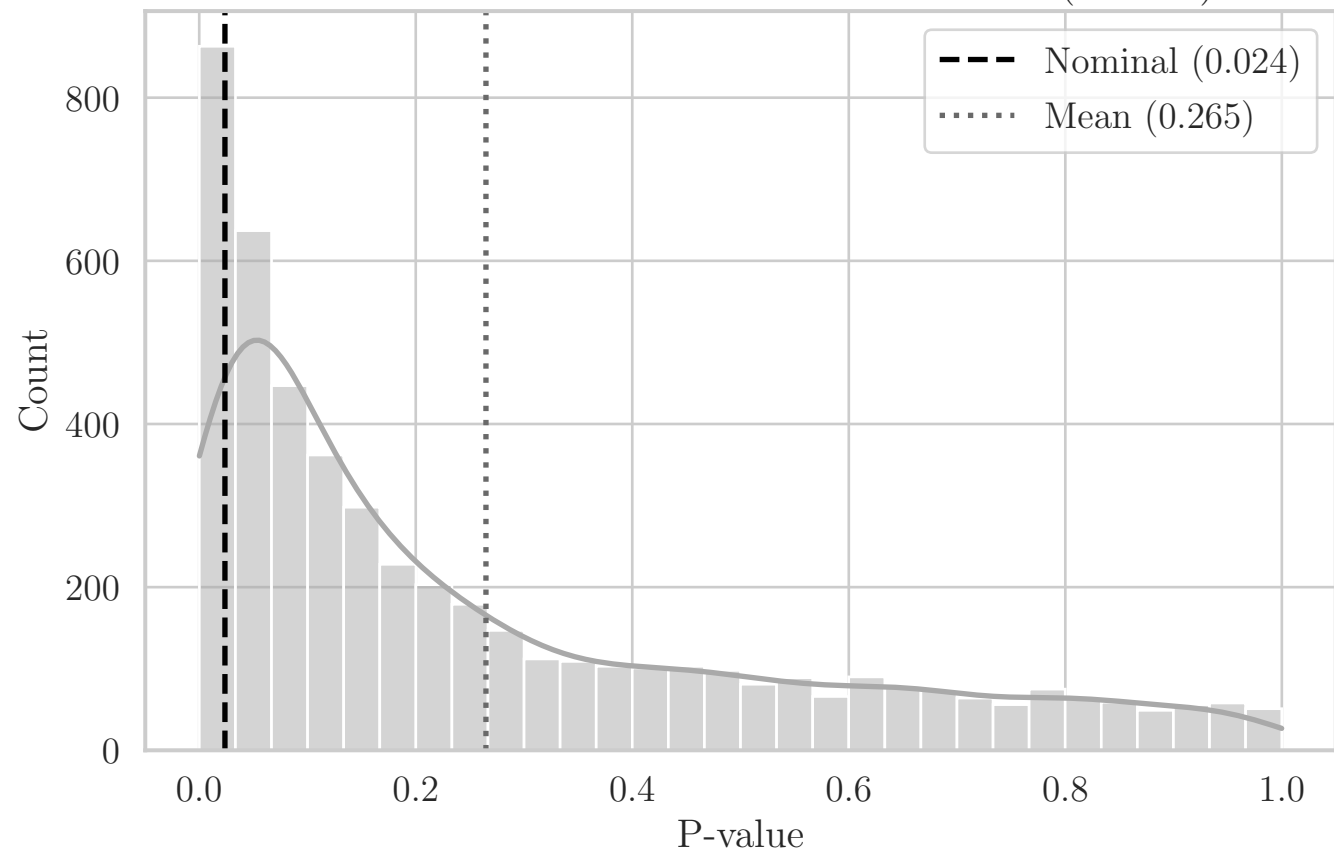
MC Distribution of P-values for ST T-Dist (F2 XY)
