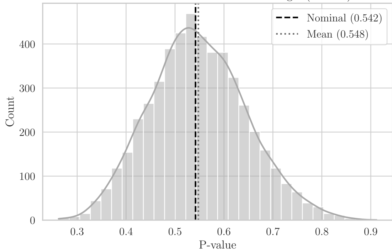
MC Distribution of P-values for T Angle (F2 XY)
