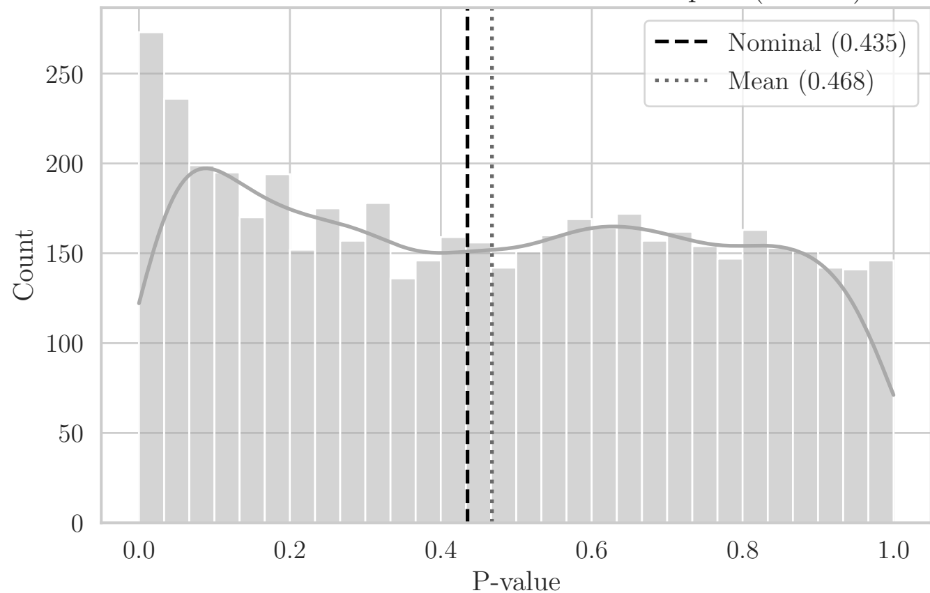
MC Distribution of P-values for ST Compact (NL YZ)
