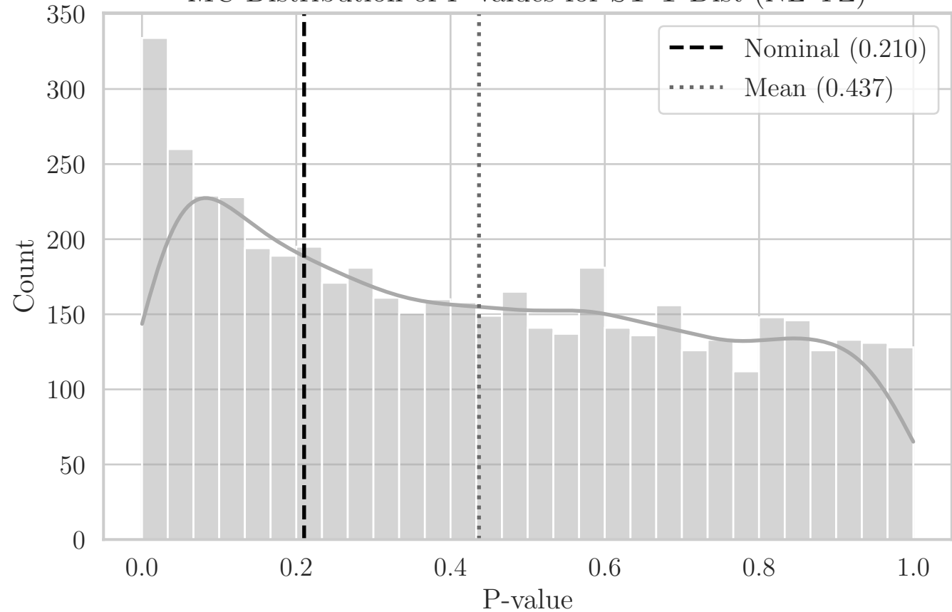
MC Distribution of P-values for ST T-Dist (NL YZ)
