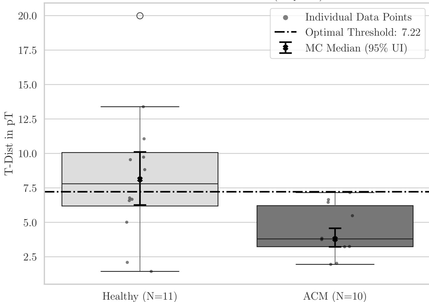
Box Plot for T T-Dist (OQ XY)
