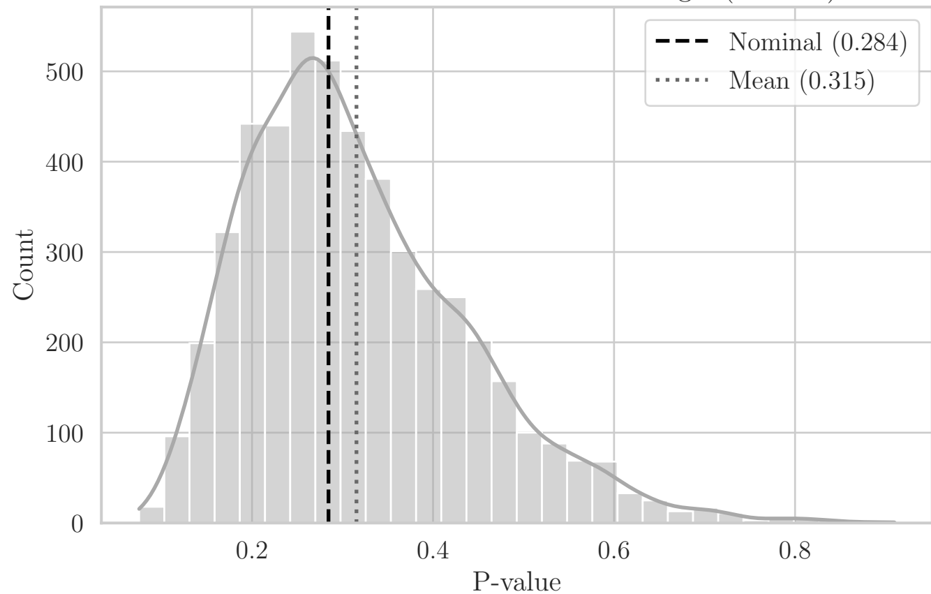
MC Distribution of P-values for T Angle (OT YZ)
