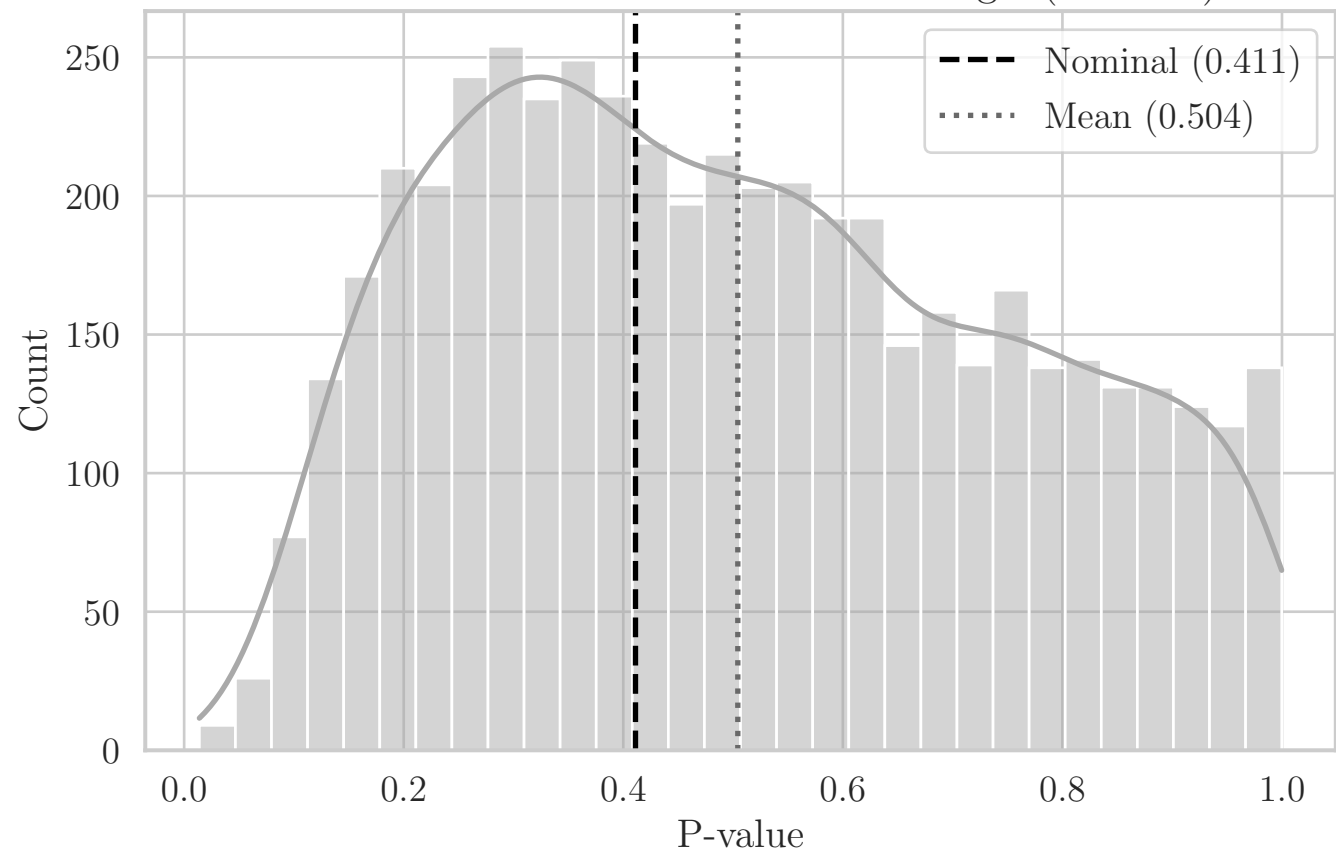
MC Distribution of P-values for ST Angle (OW YZ)
