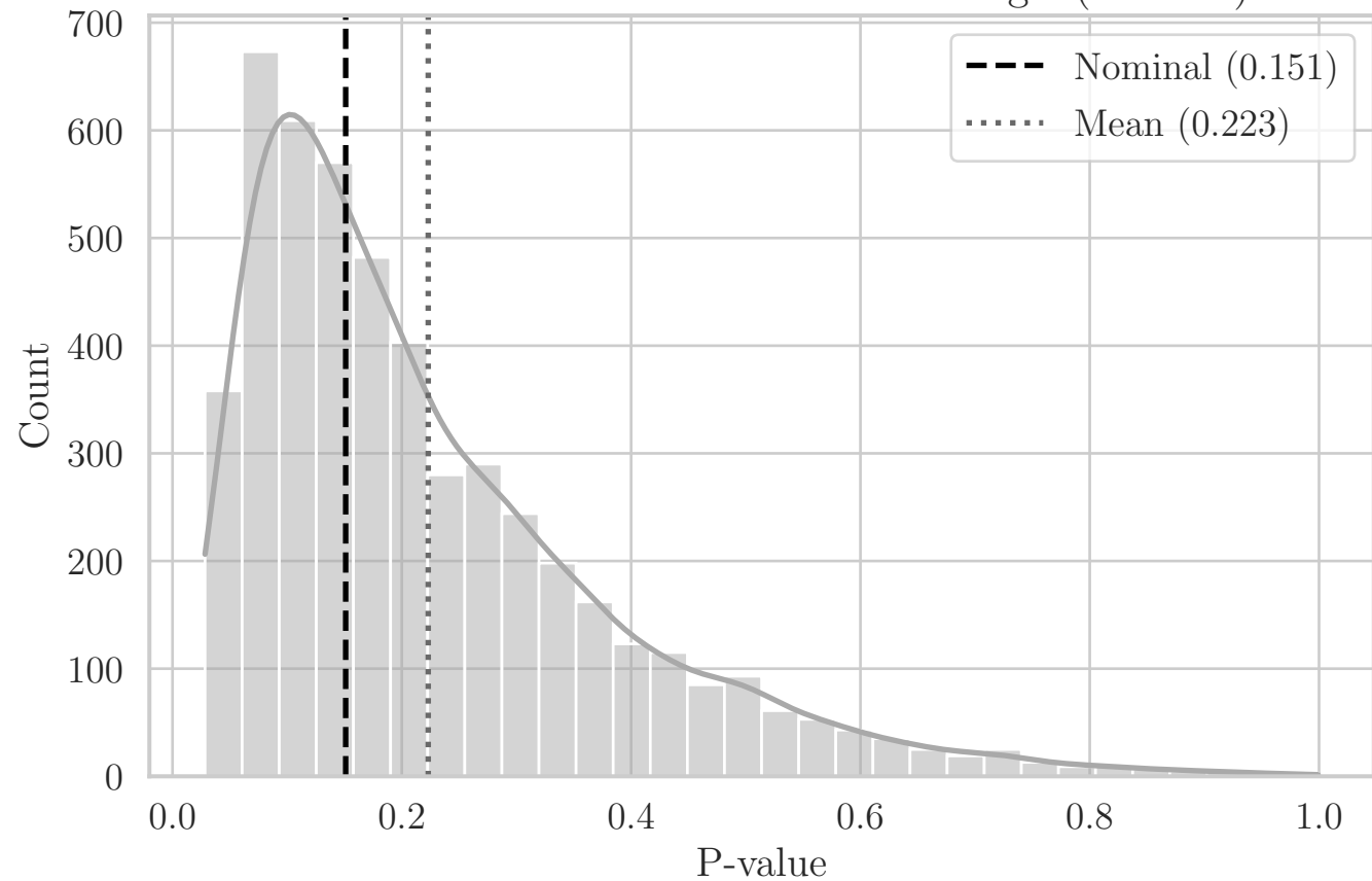
MC Distribution of P-values for ST Angle (OX XY)
