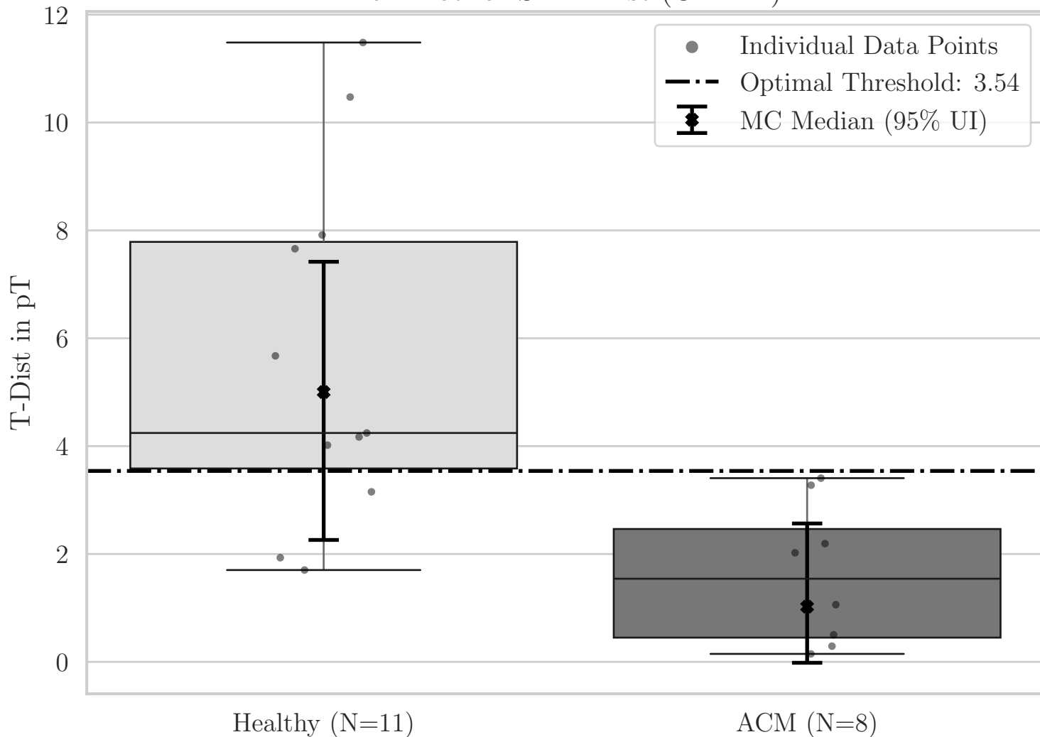
Box Plot for ST T-Dist (OX XY)
