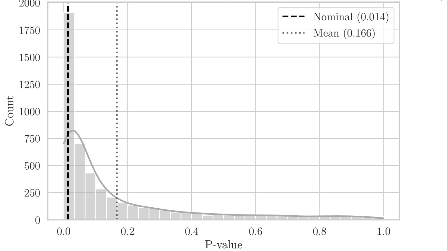
MC Distribution of P-values for ST Area (Aggregated Bottom-Left Quadrant XY)
