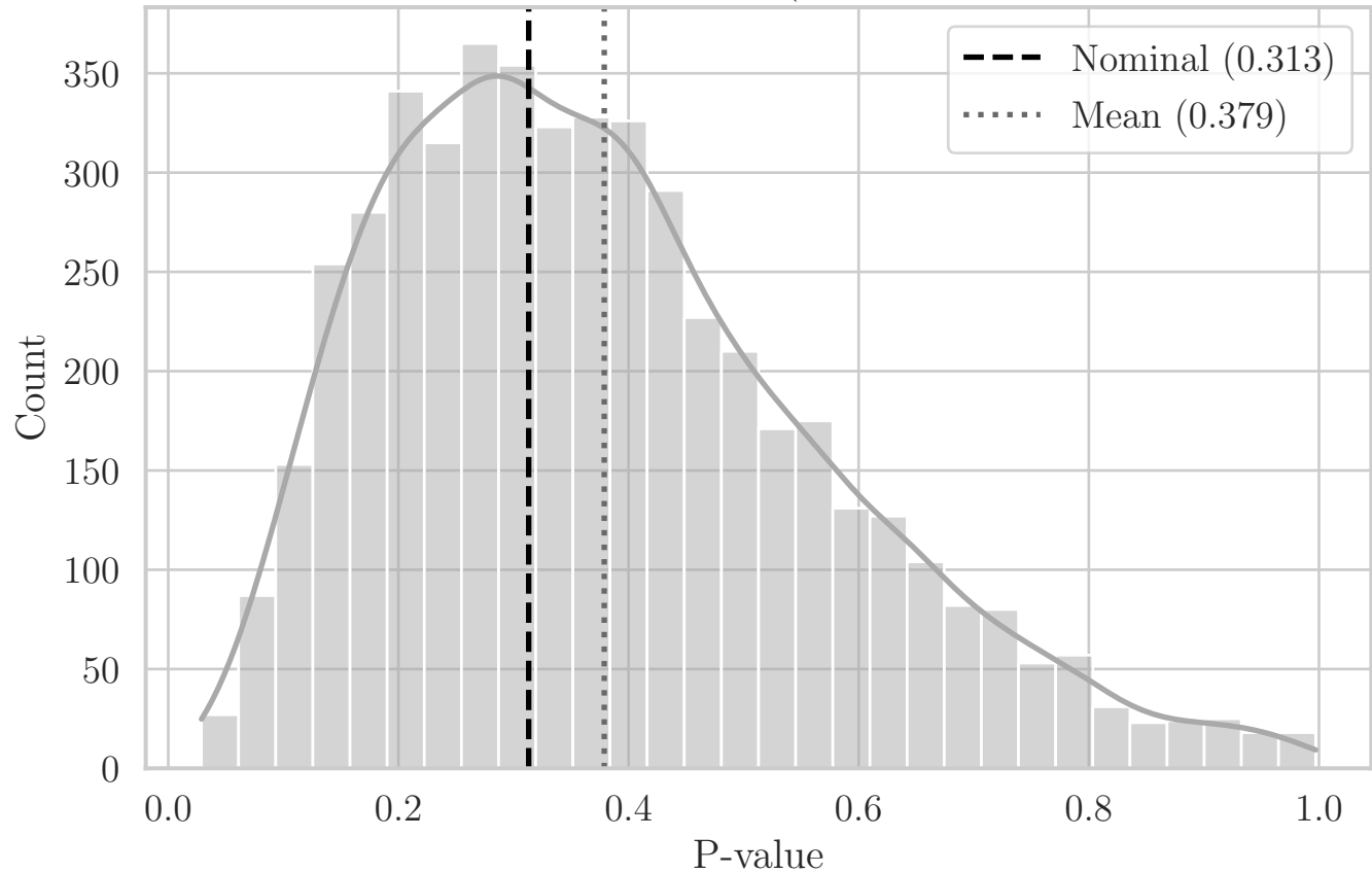
MC Distribution of P-values for QRS Angle (Aggregated Bottom-Right Quadrant YZ)
