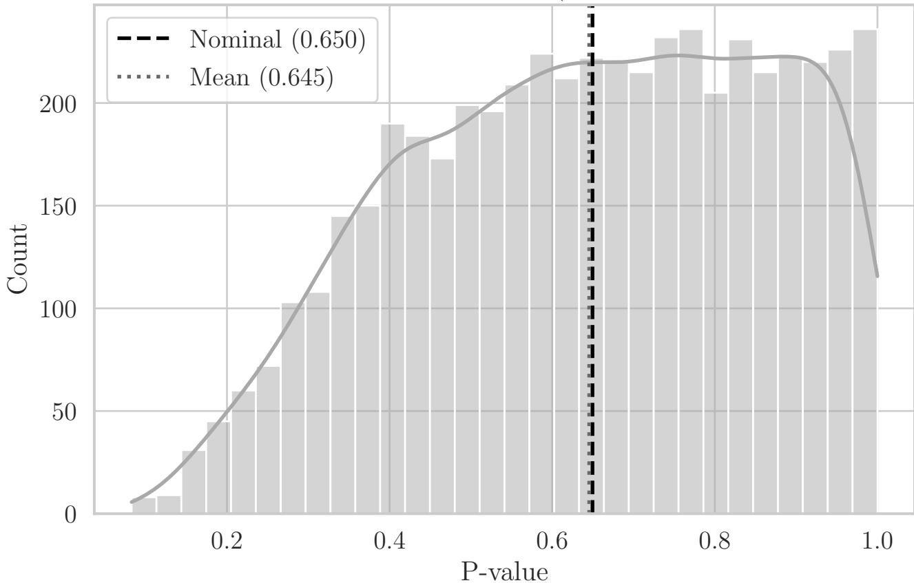
MC Distribution of P-values for QRS Angle (Aggregated Top-Left Quadrant YZ)
