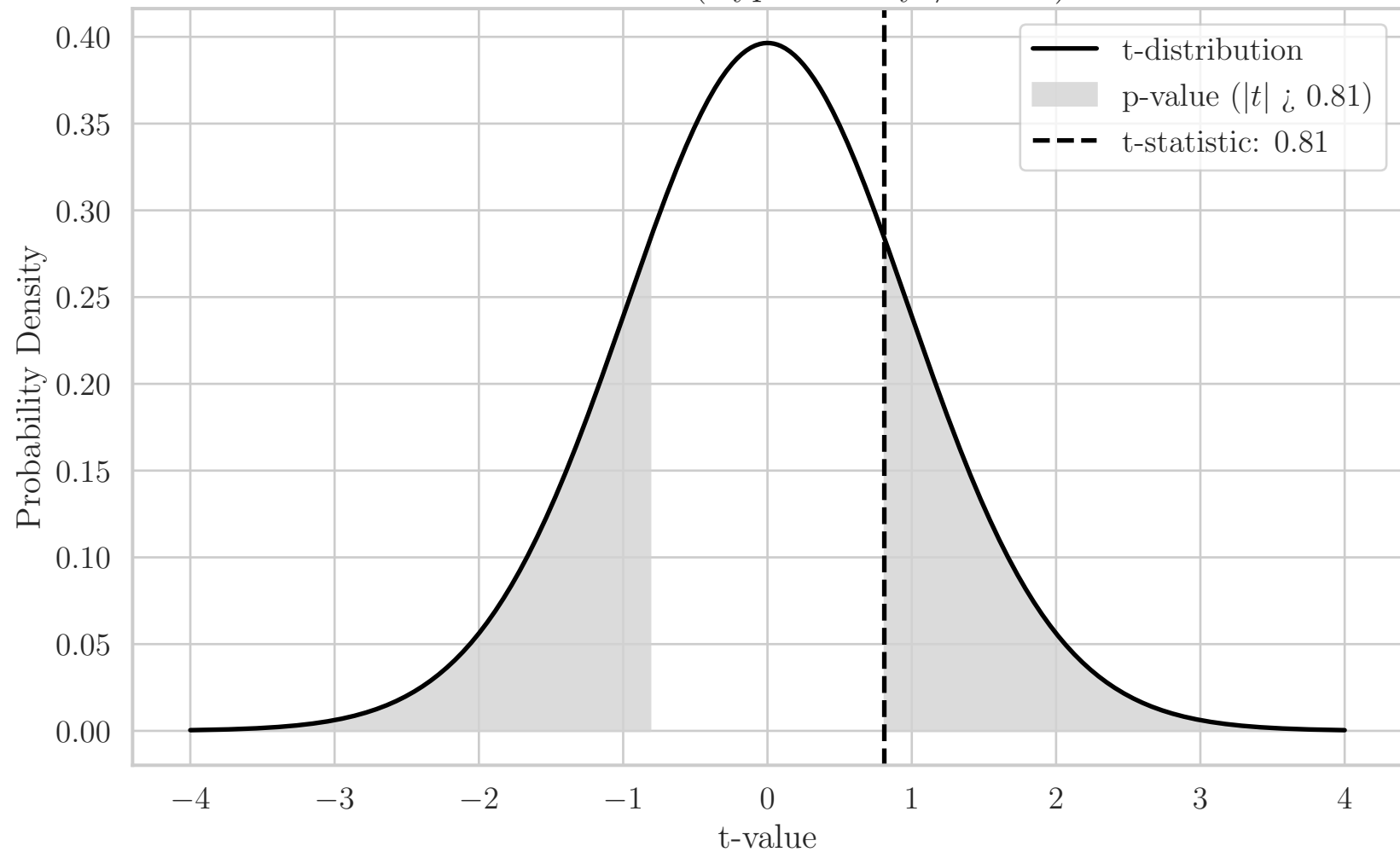
t-Distribution (Hyp: Healthy \neq ACM)
