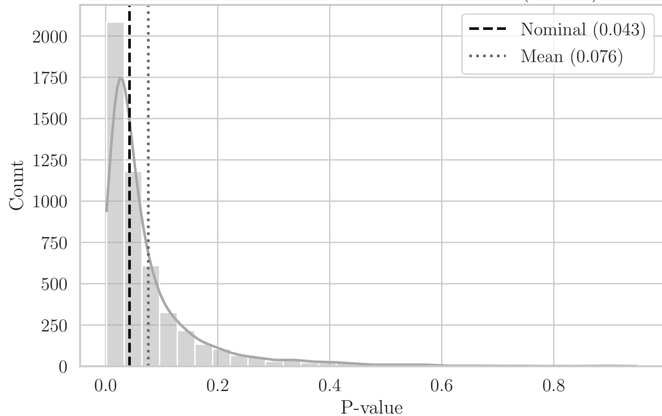
MC Distribution of P-values for T T-Dist (C1 XY)
