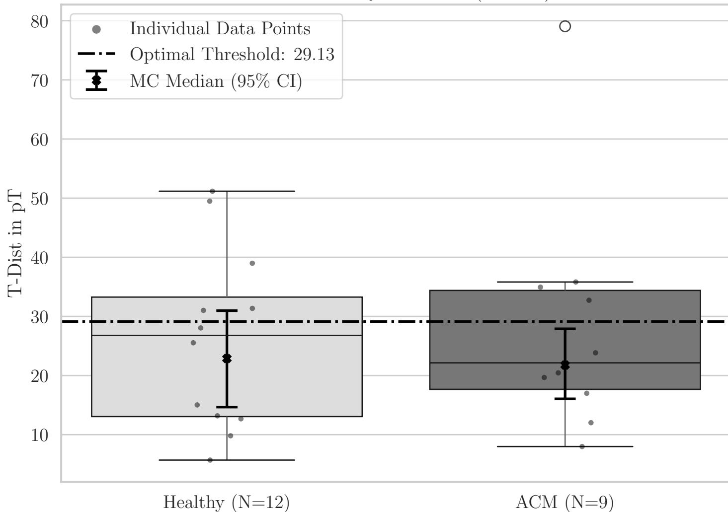
Box Plot for QRS T-Dist (EZ YZ)
