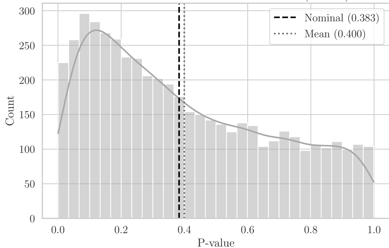
MC Distribution of P-values for ST Area (EZ YZ)
