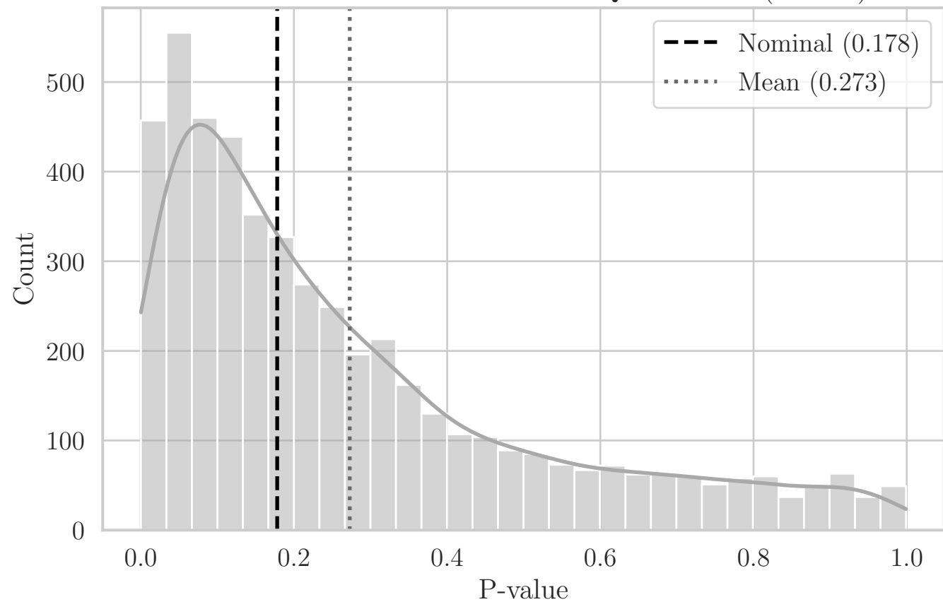
MC Distribution of P-values for QRS T-Dist (F0 YZ)
