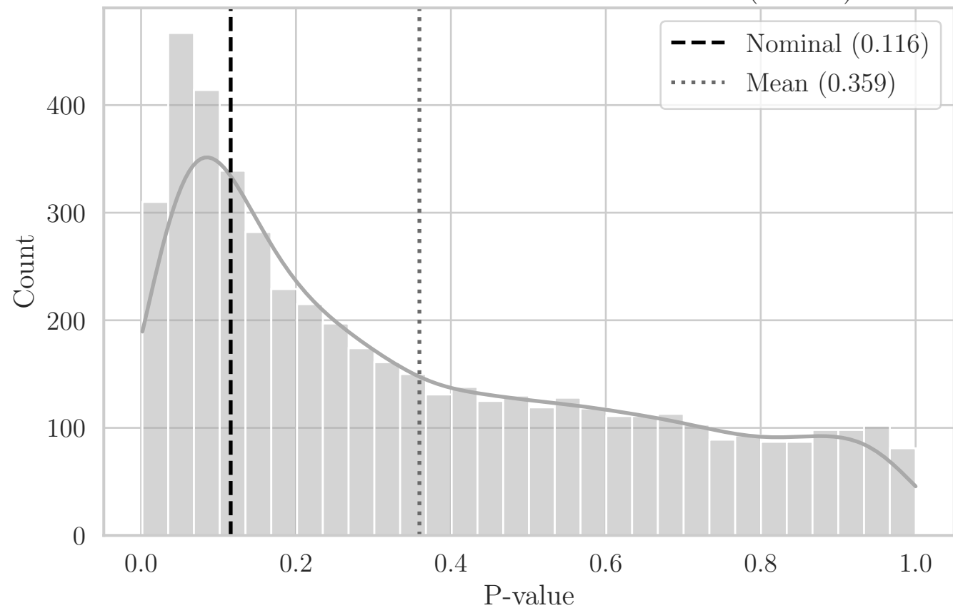
MC Distribution of P-values for ST Area (F0 YZ)
