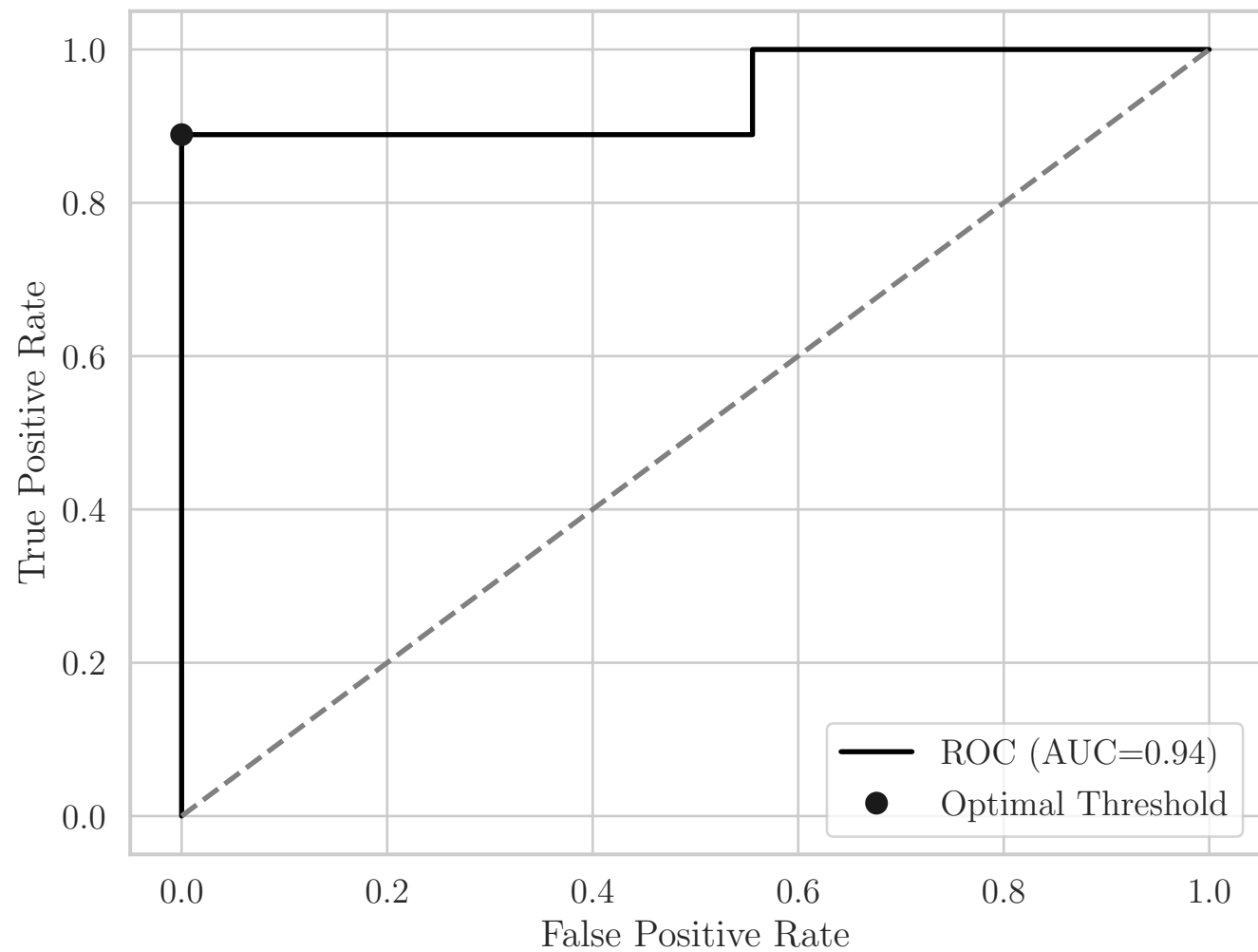
ROC Curve
