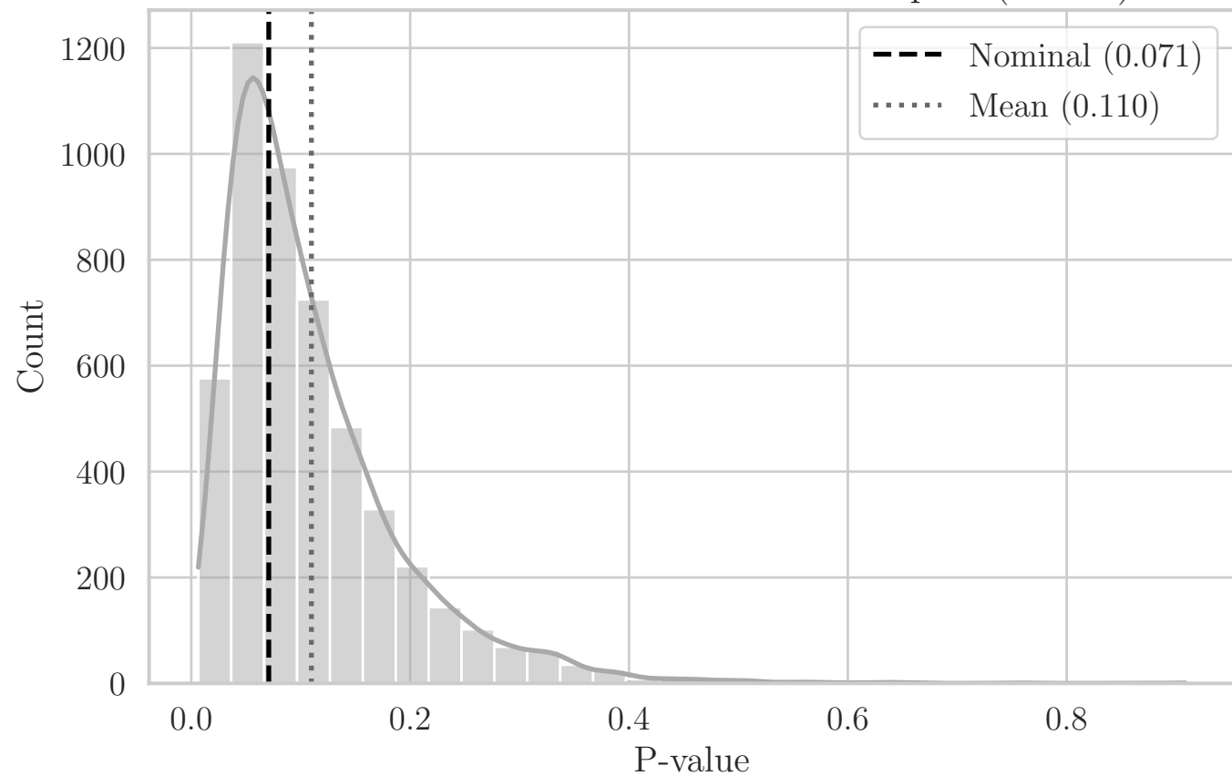
MC Distribution of P-values for T Compact (F0 YZ)
