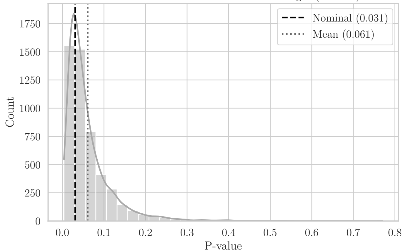
MC Distribution of P-values for ST Angle (F2 XY)
