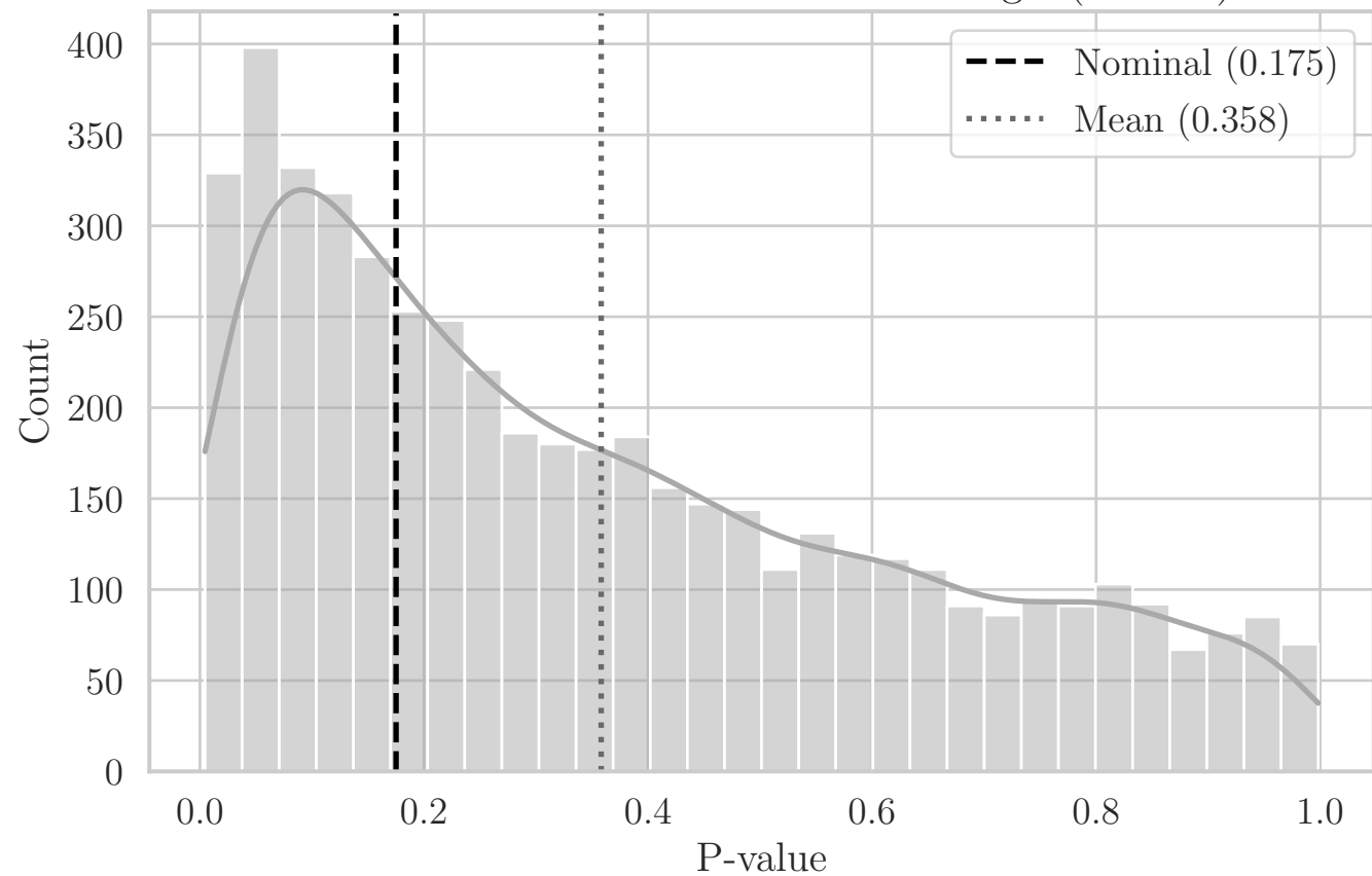
MC Distribution of P-values for T Angle (NL YZ)
