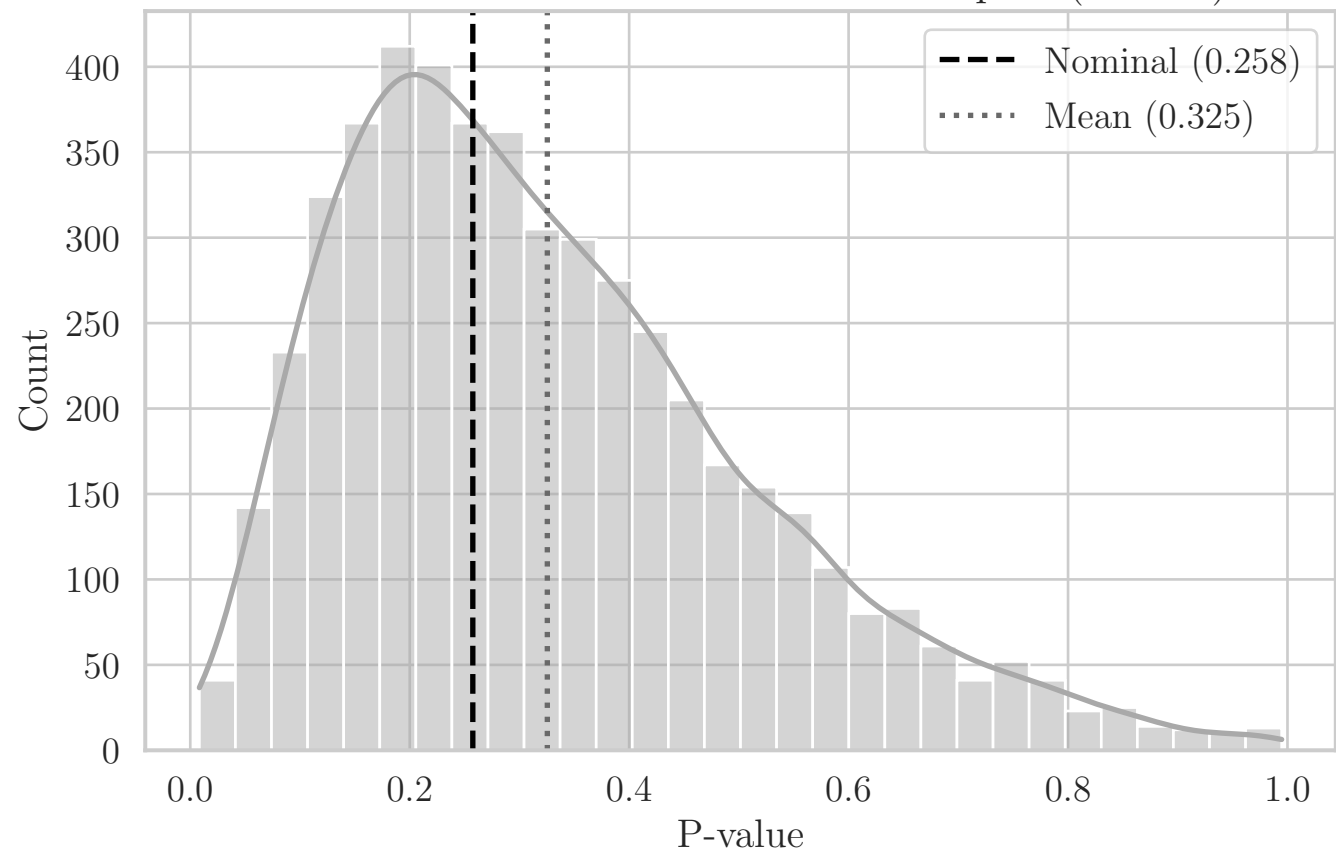
MC Distribution of P-values for T Compact (NL YZ)
