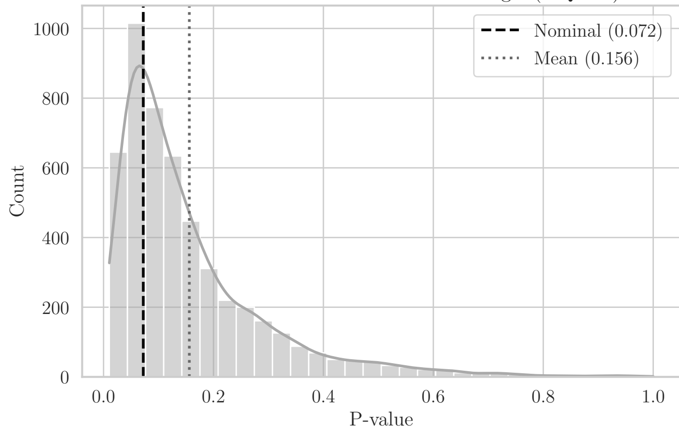
MC Distribution of P-values for ST Angle (OQ XY)
