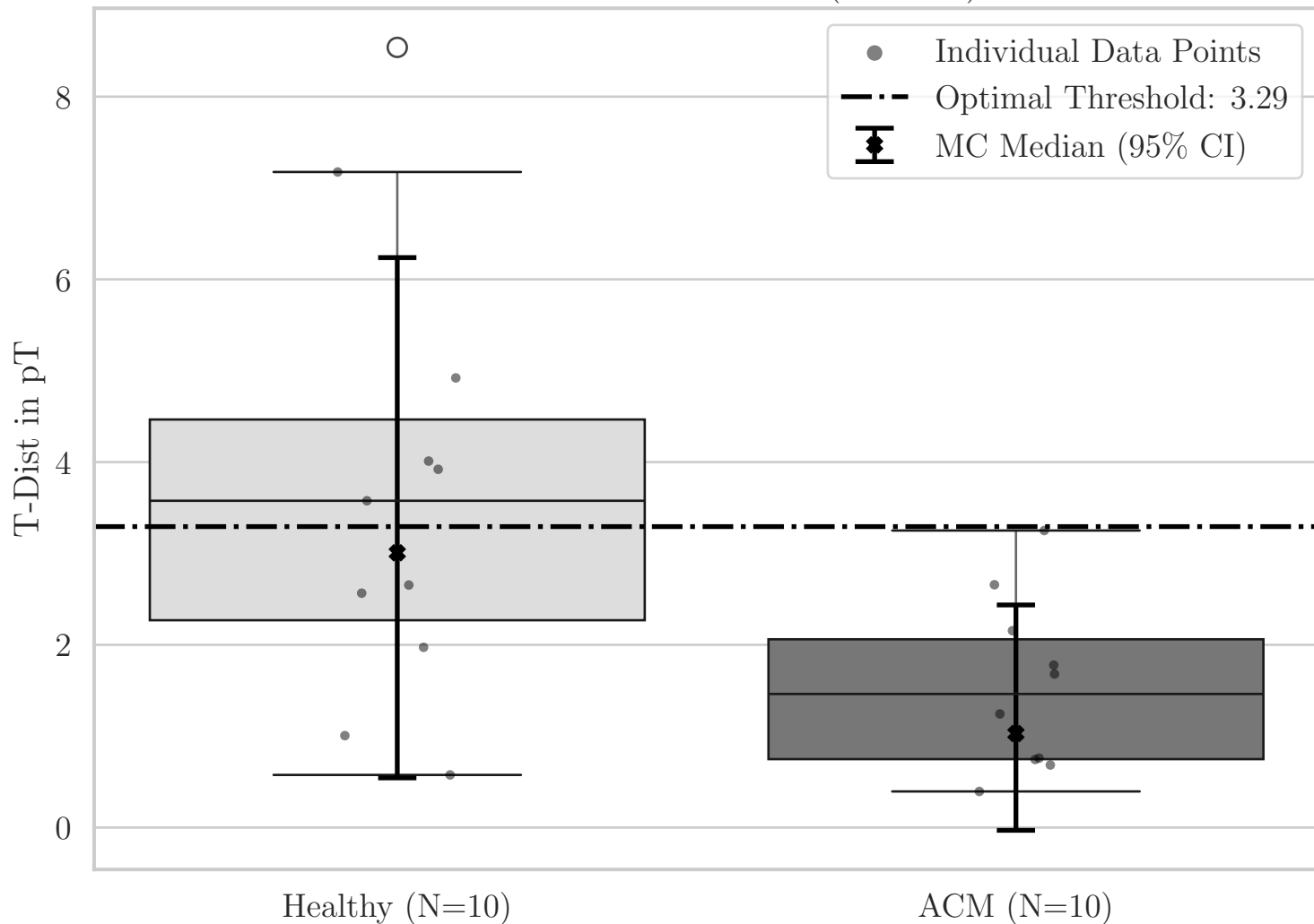
Box Plot for ST T-Dist (OR XY)
