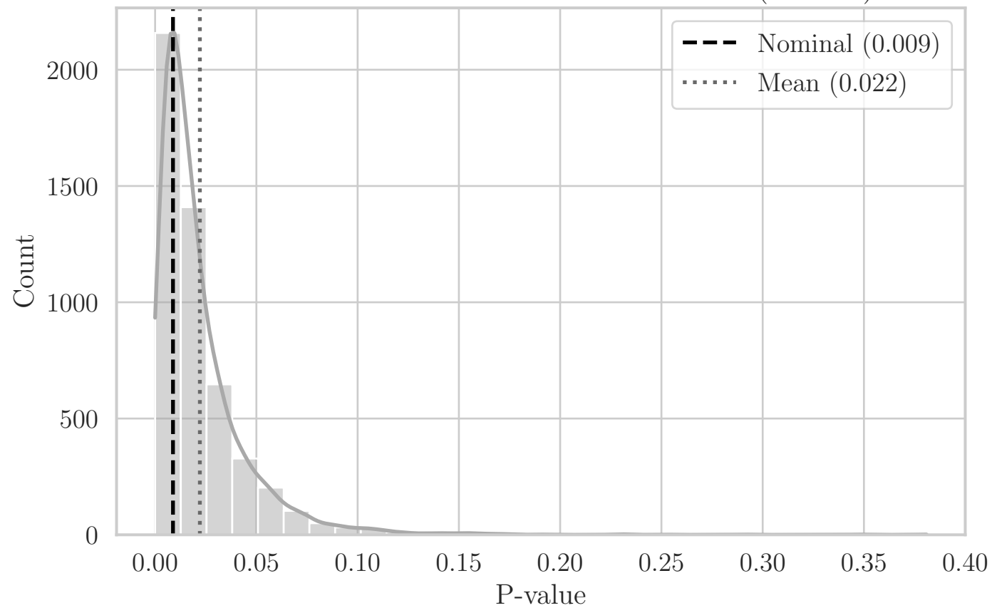
MC Distribution of P-values for T T-Dist (OT YZ)
