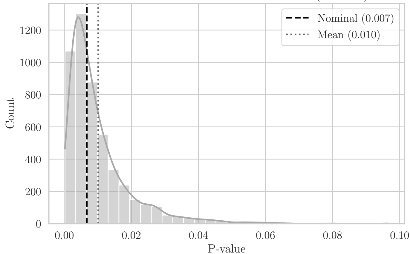
MC Distribution of P-values for T T-Dist (OW YZ)
