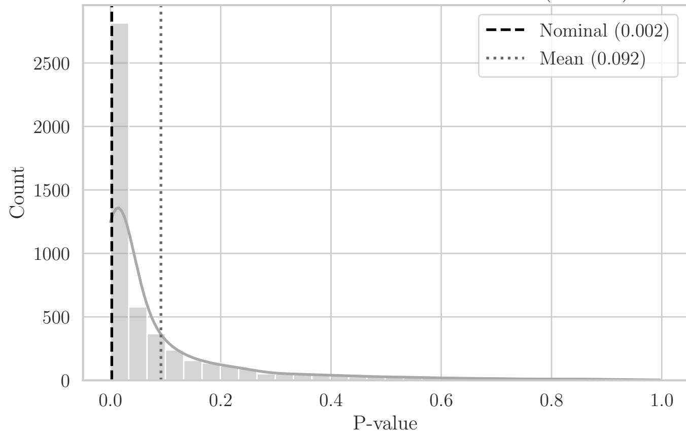
MC Distribution of P-values for ST T-Dist (OX XY)
