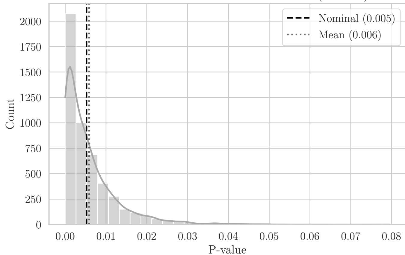
MC Distribution of P-values for T T-Dist (OX XY)
