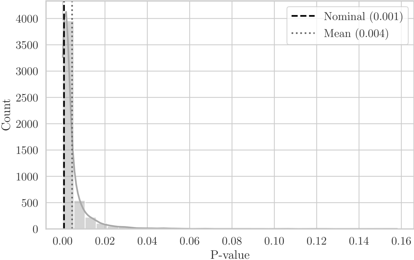
MC Distribution of P-values for QRS T-Dist (Aggregated Bottom-Left Quadrant XY)
