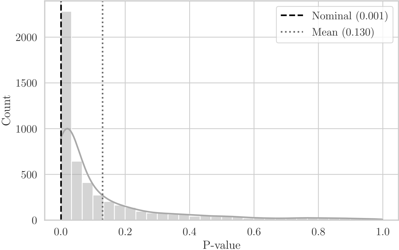
MC Distribution of P-values for ST T-Dist (Aggregated Bottom-Left Quadrant XY)
