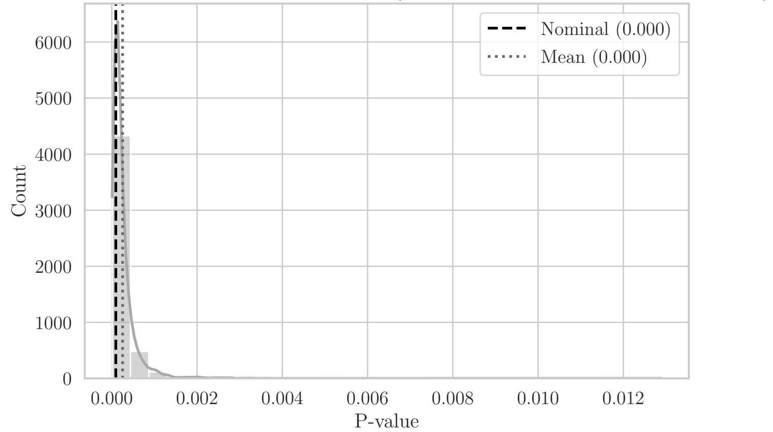
MC Distribution of P-values for T T-Dist (Aggregated Bottom-Left Quadrant XY)
