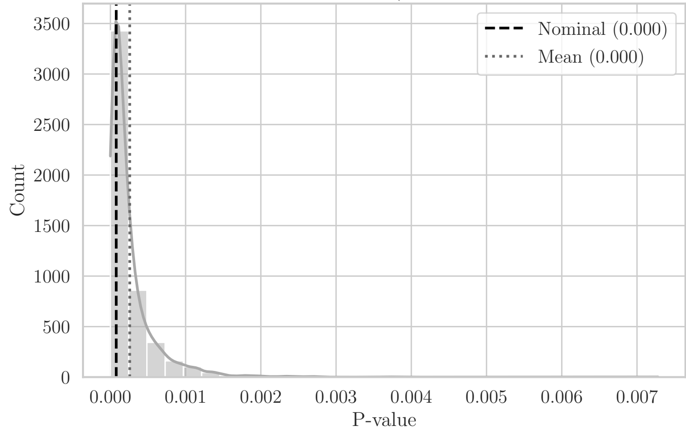
MC Distribution of P-values for T T-Dist (Aggregated Bottom-Left Quadrant YZ)
