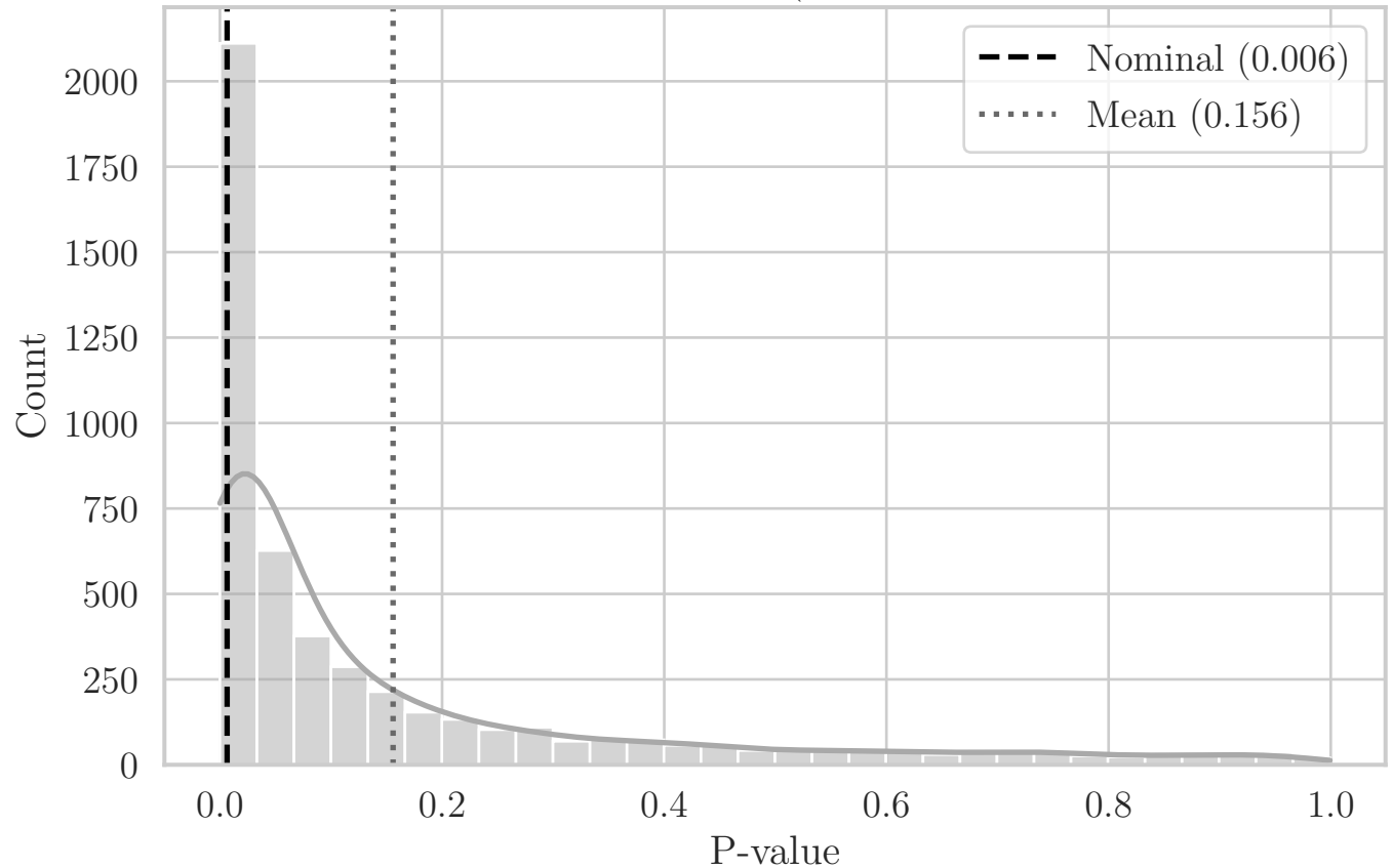
MC Distribution of P-values for ST T-Dist (Aggregated Bottom-Right Quadrant XY)
