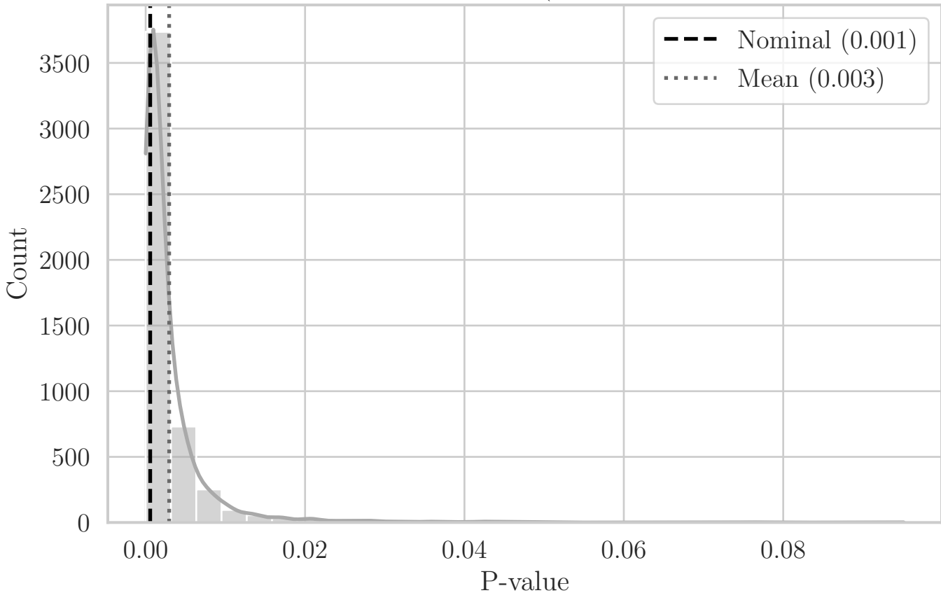
MC Distribution of P-values for T Compact (Aggregated Bottom-Right Quadrant XY)
