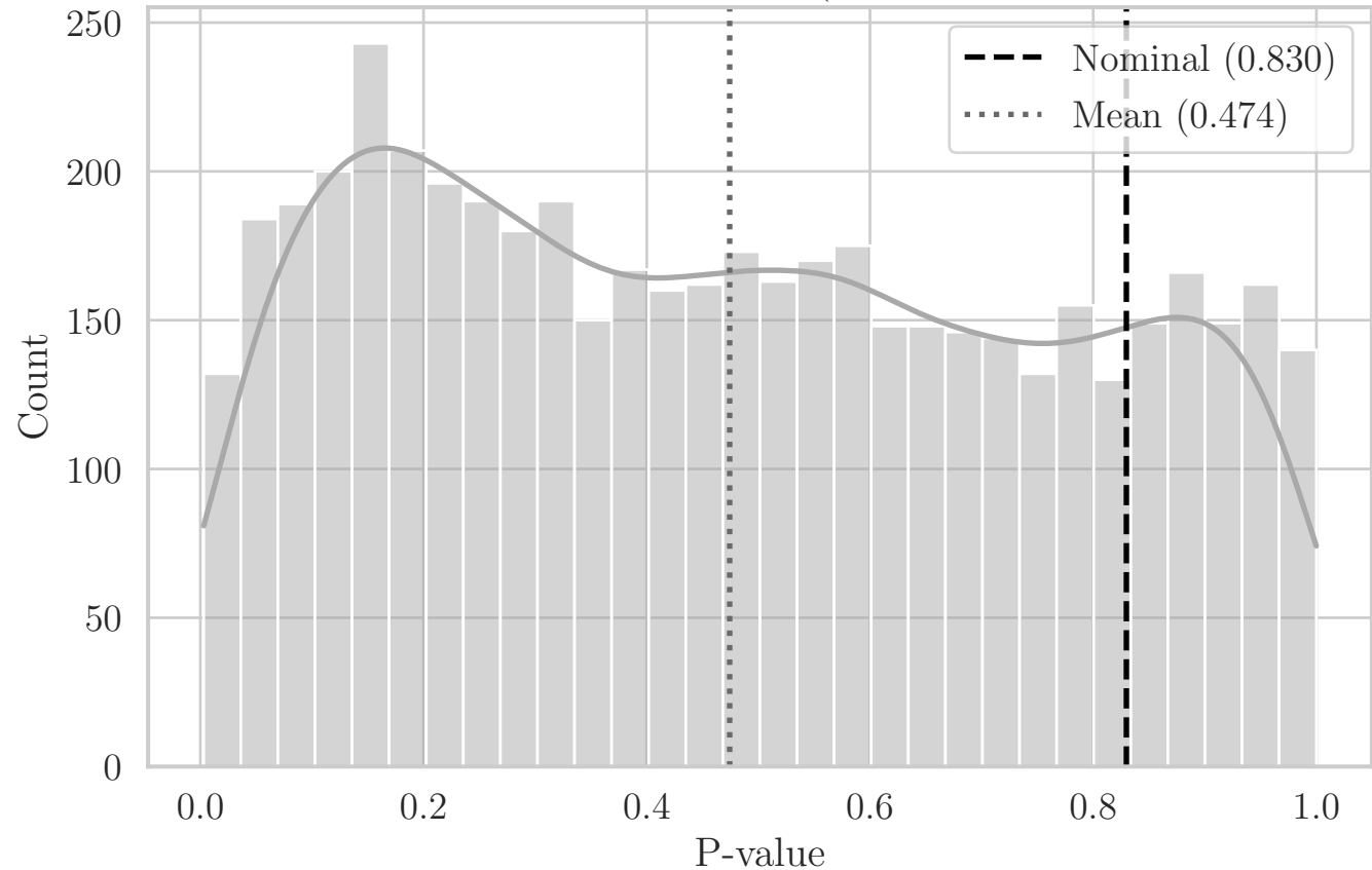
MC Distribution of P-values for QRS Compact (Aggregated Bottom-Right Quadrant YZ)
