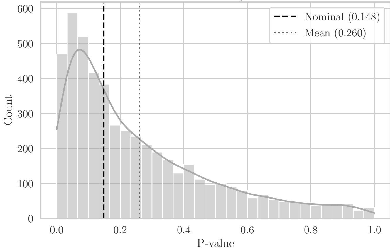
MC Distribution of P-values for QRS T-Dist (Aggregated Top-Left Quadrant XY)
