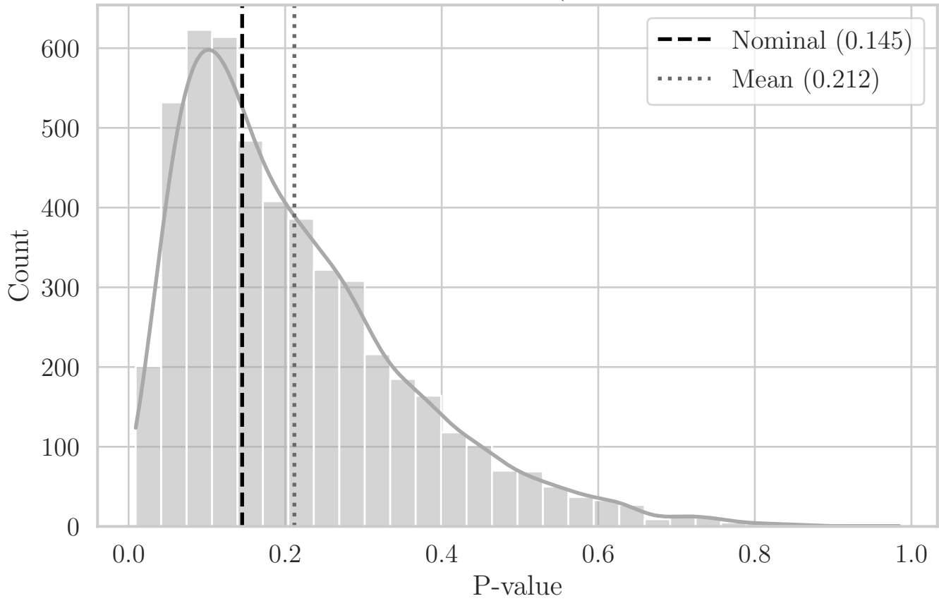
MC Distribution of P-values for ST Angle (Aggregated Top-Left Quadrant XY)
