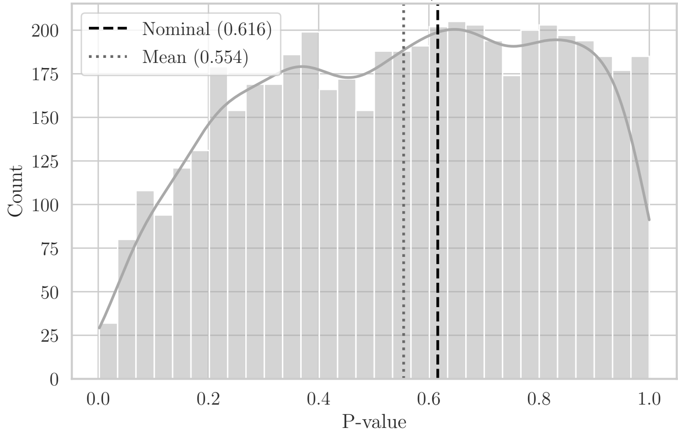
MC Distribution of P-values for QRS Compact (Aggregated Top-Left Quadrant YZ)
