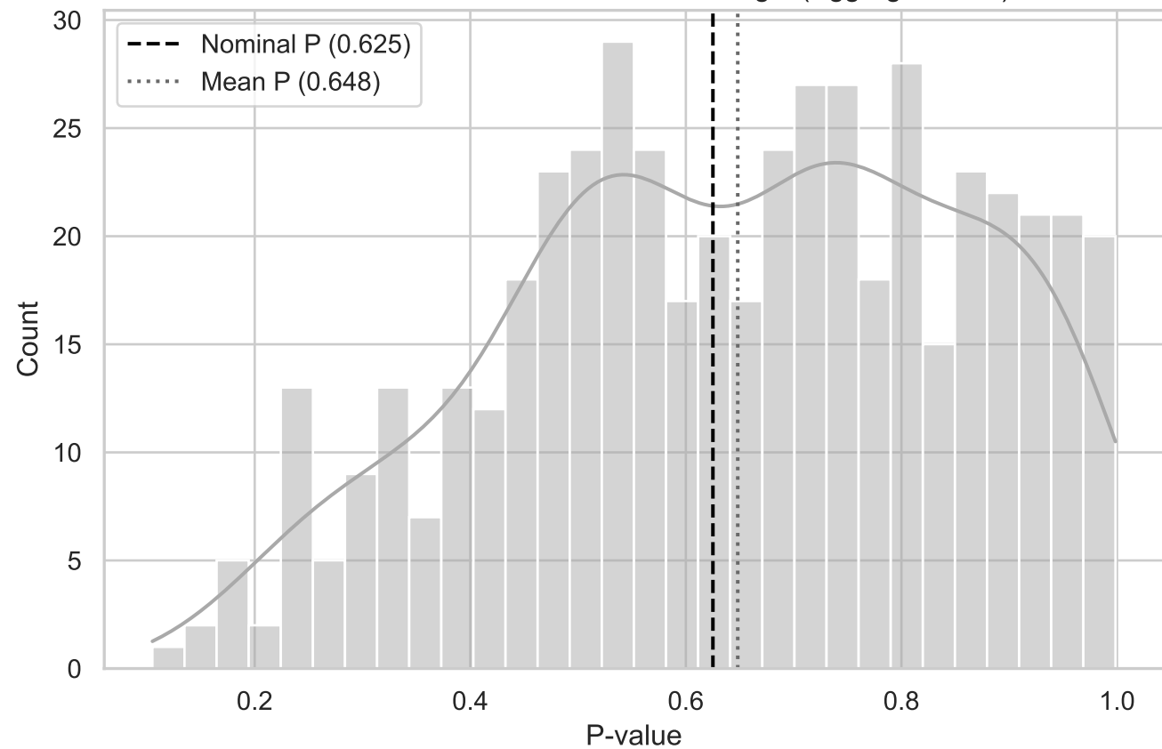
MC Distribution of P-values for QRS Angle (Aggregated YZ)
