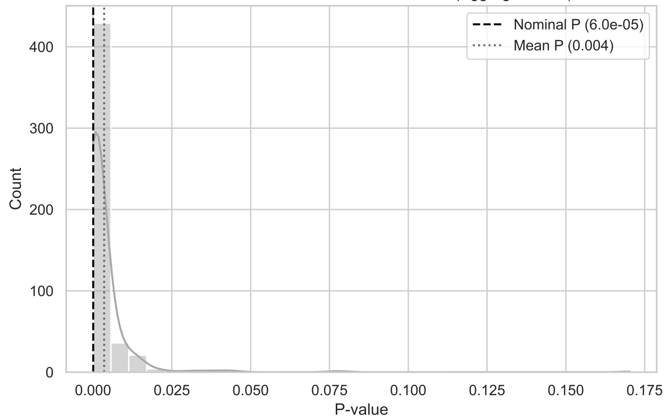
MC Distribution of P-values for QRS T-Dist (Aggregated XY)
