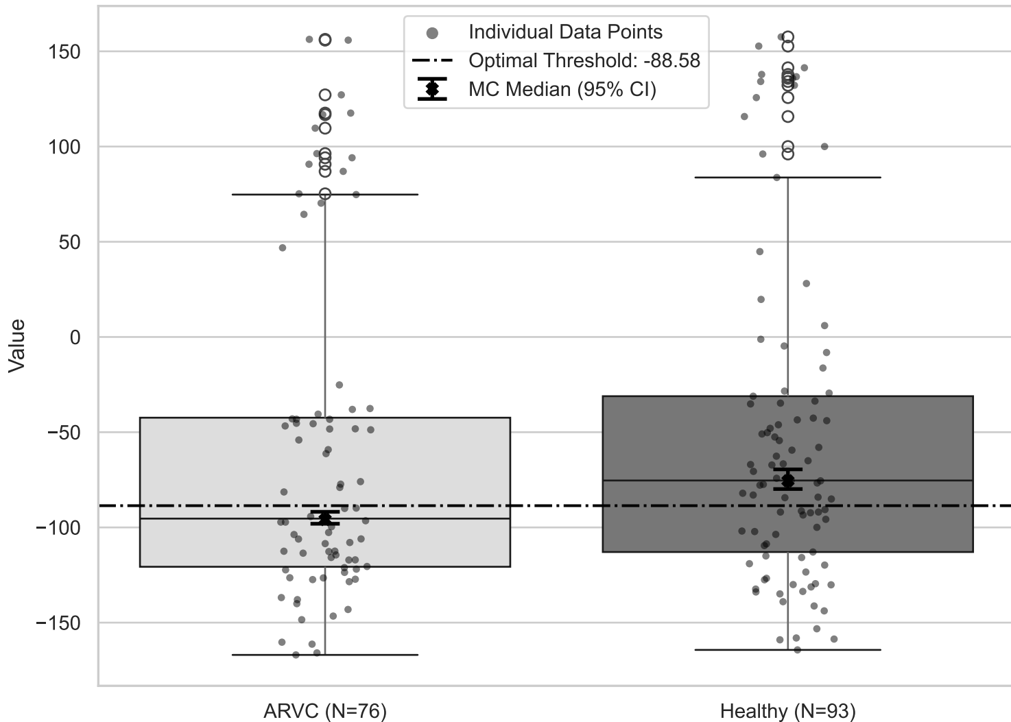
Box Plot of Nominal Data with MC Medians for T Angle (Aggregated XY)
