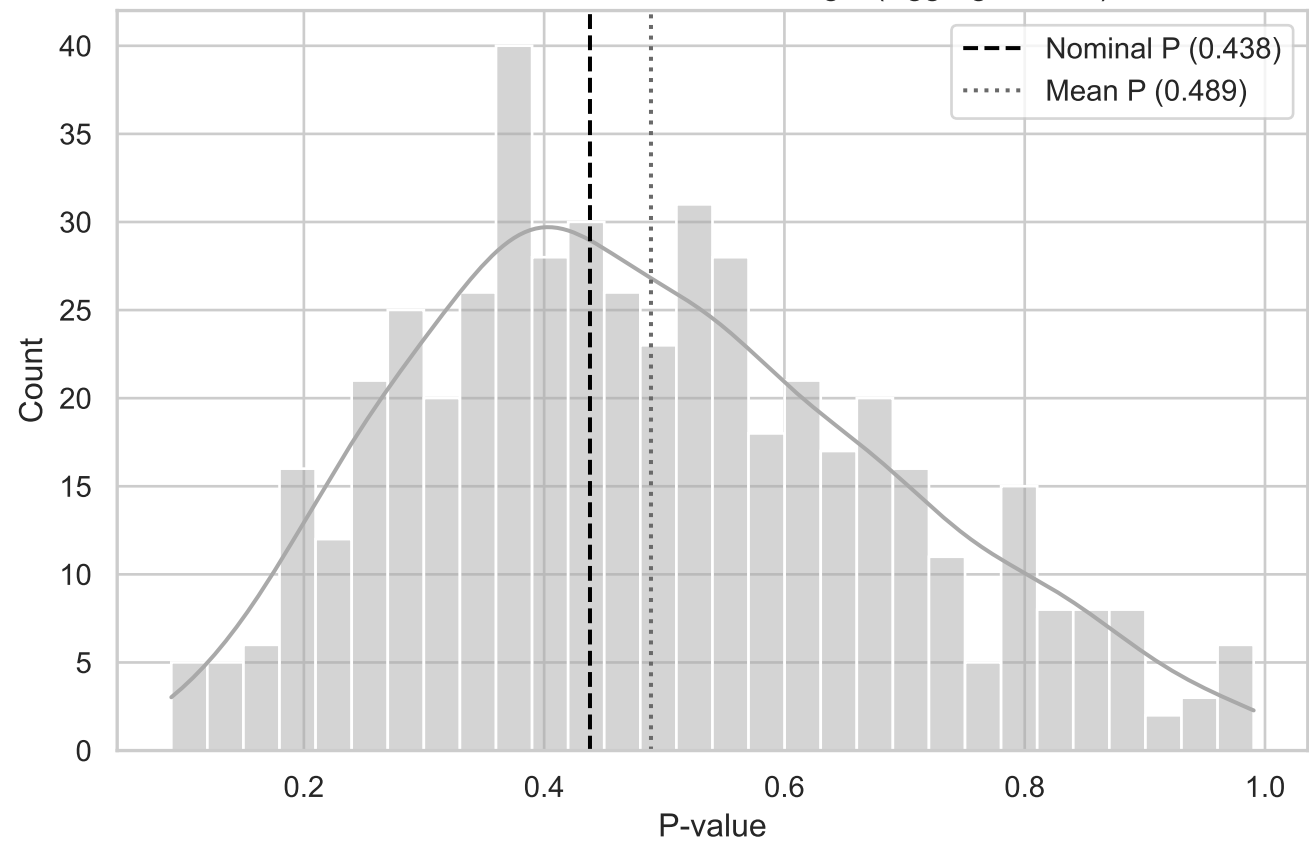
MC Distribution of P-values for T Angle (Aggregated YZ)
