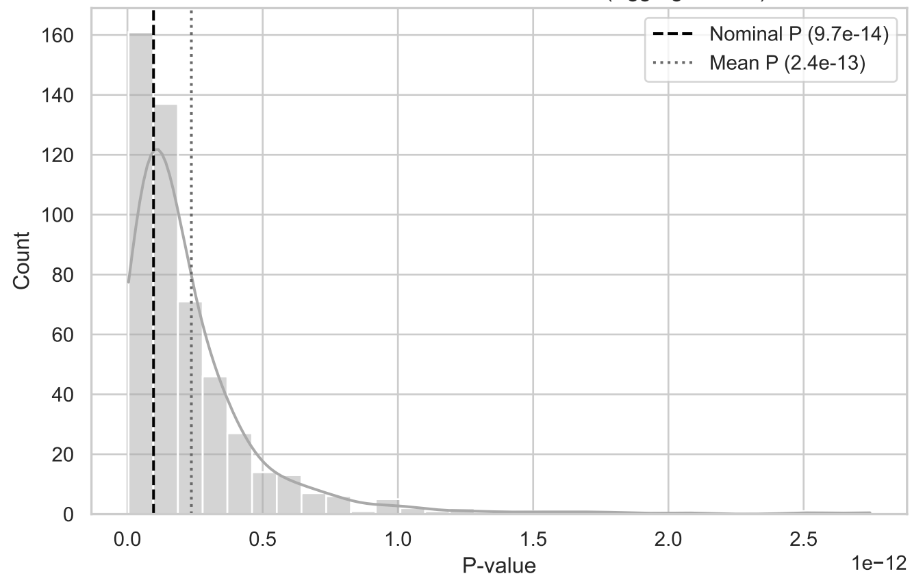
MC Distribution of P-values for T Area (Aggregated YZ)
