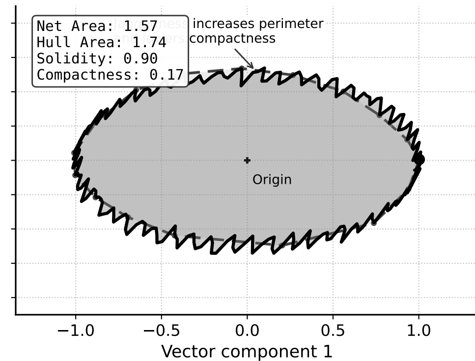
Fragmented / jagged loop
