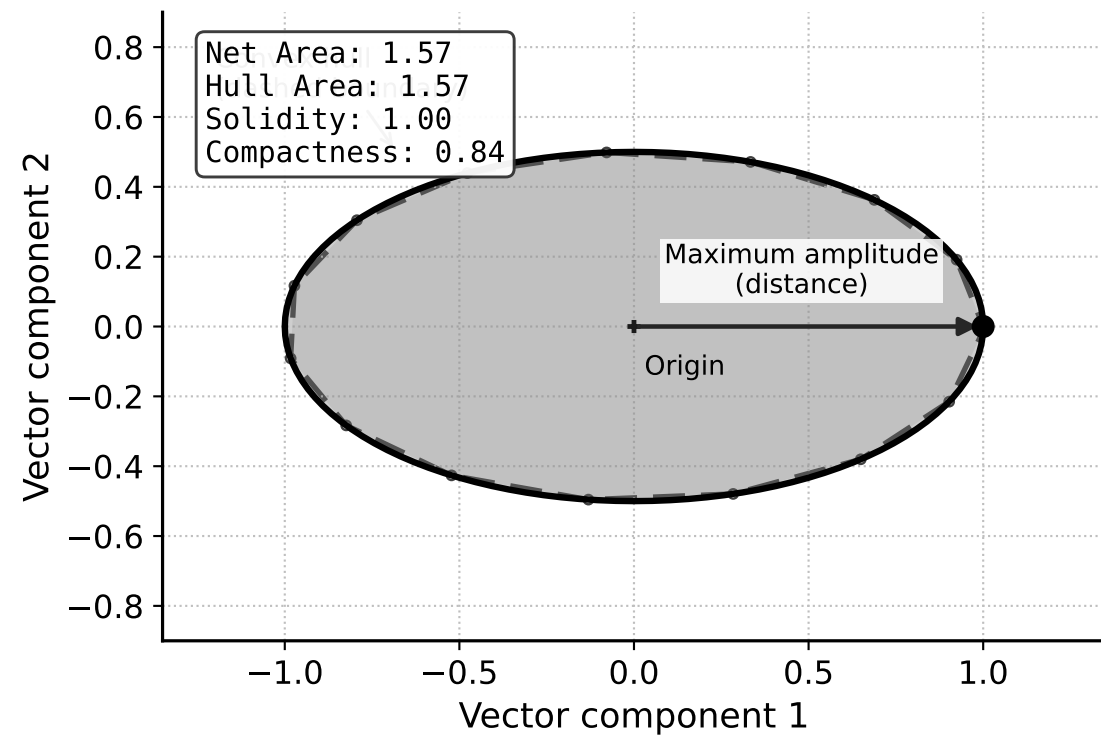
Smooth elliptic loop
