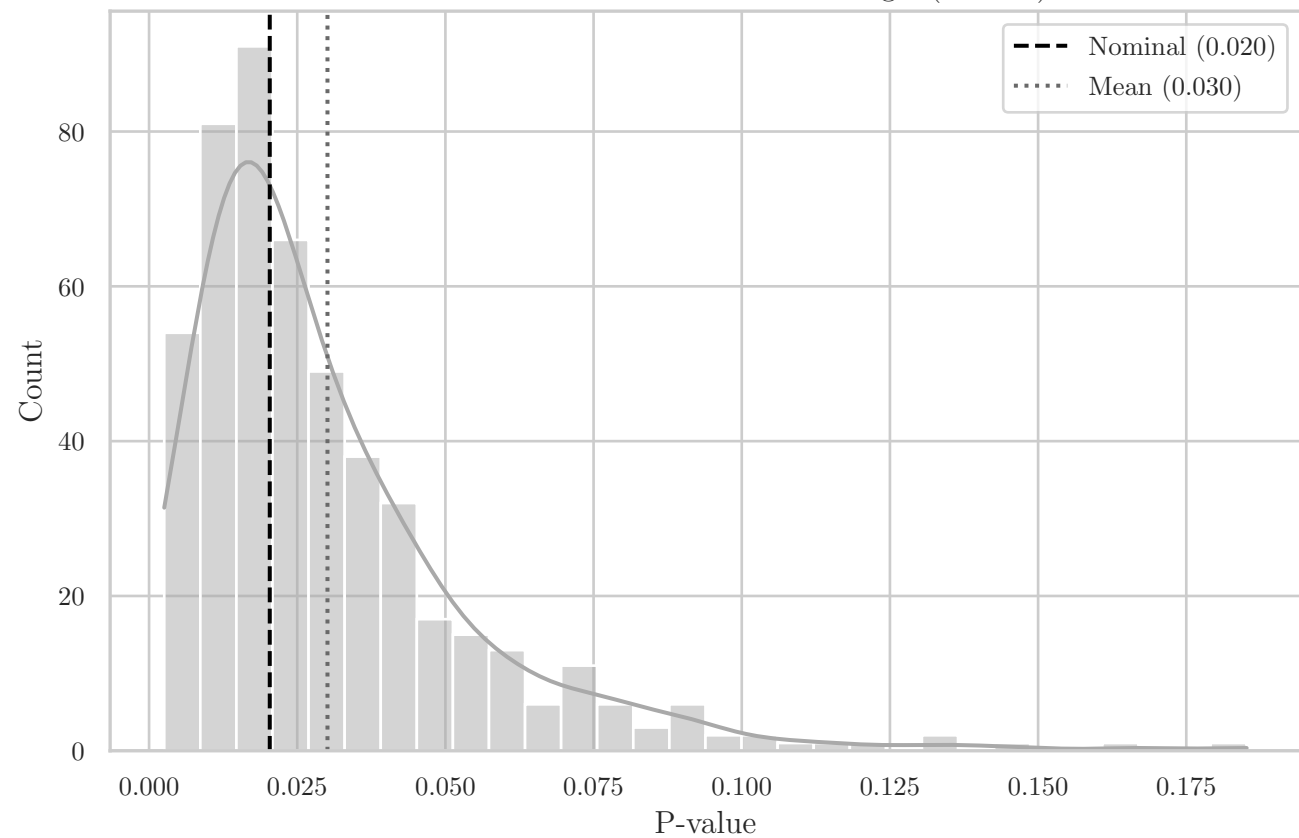
MC Distribution of P-values for T Angle (C1 XY)
