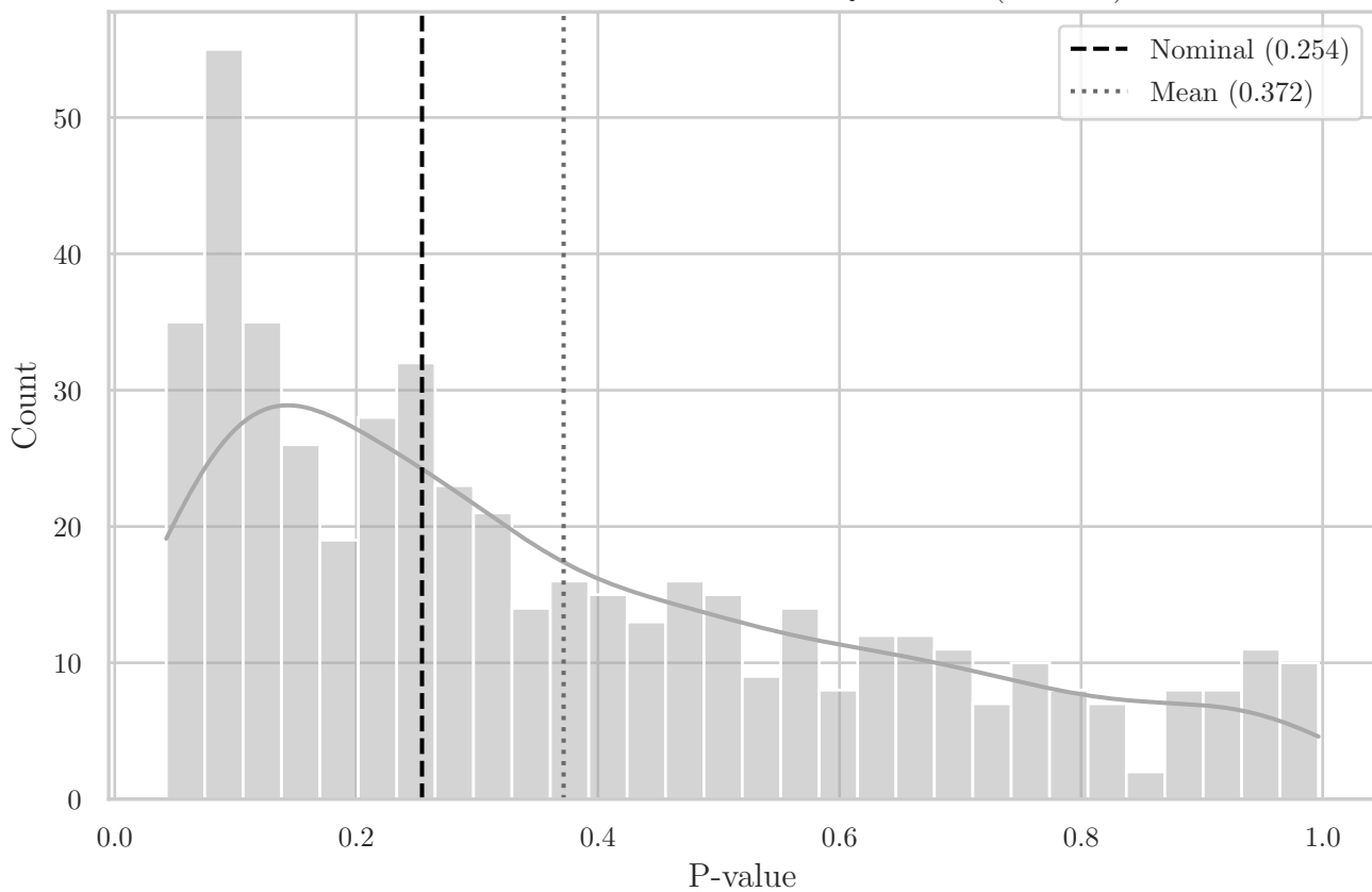
MC Distribution of P-values for QRS Area (EY XY)
