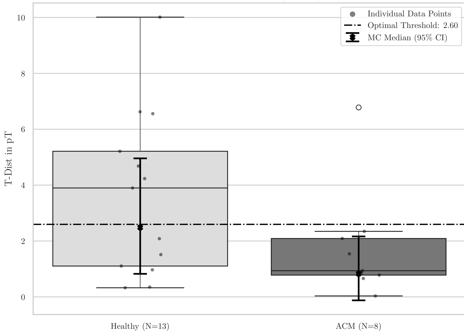
Box Plot for ST T-Dist (EY XY)
