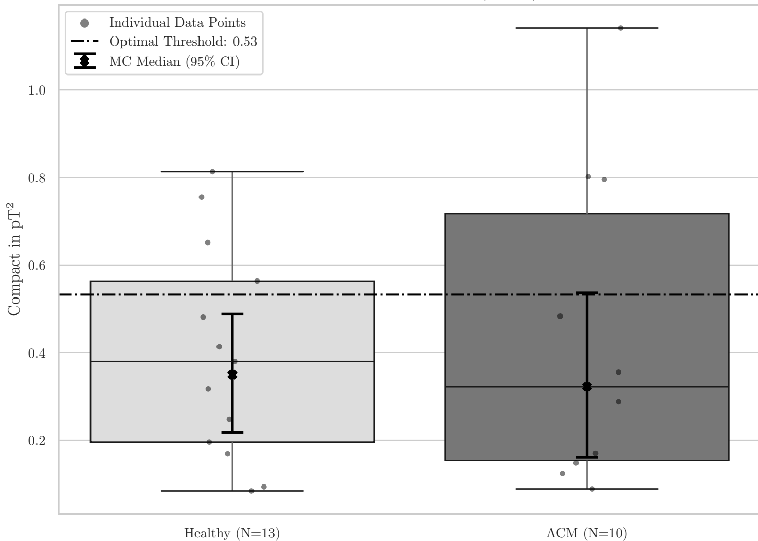
Box Plot for QRS Compact (F1 YZ)
